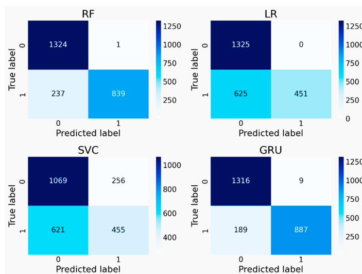
Figure 5: RF's, LR's, SVC's, and GRU's Confusion matrix from real dataset. (Reproduced from [10]).
