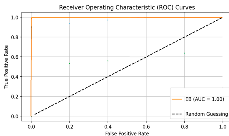
Figure 4: EB approach's ROC from the actual dataset (AUC = 1.00). (Reproduced from [10]).
